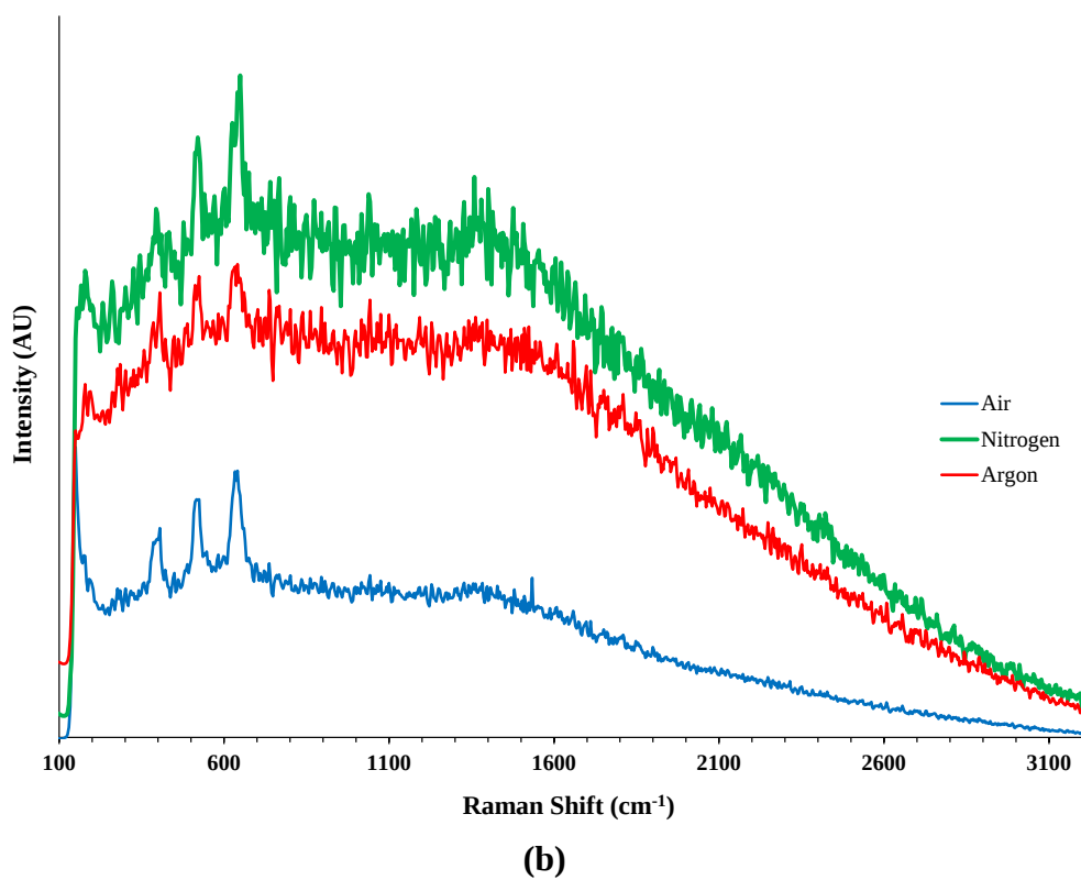
Figure S2. Raman confocal laser spectra of \text{TiO}_2 nanostructures anodized at 0 rpm (a) and 2500 rpm (b) and annealed in different atmospheres (air, nitrogen and argon).
