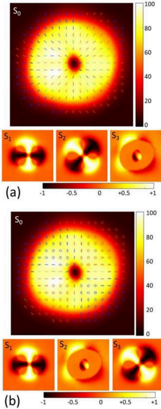
Fig. 5. Images of the experimental Stokes parameters for the vector beams in (a) Figure 3 and (b) Figure 4. S_1 , S_2 and S_3 are normalized Stokes parameters.
