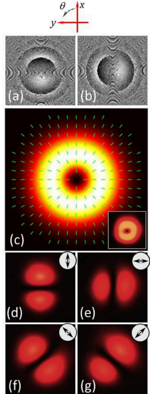
Fig. 3. (a)-(b) Central part of the phase-only holograms displayed on LCoS1 and LCoS2 to generate HG_{10} and HG_{01} modes. (c) Expected polarization pattern (the inset shows the CCD capture without analyzer). Experimental result with a linear analyzer oriented (d) vertical ( HG_{10} ), (e) horizontal ( HG_{01} ), (f) at 45^\circ ( HG_D ) and (g) at -45^\circ ( HG_A ). The analyzer's orientation is indicated on the top of each picture.
