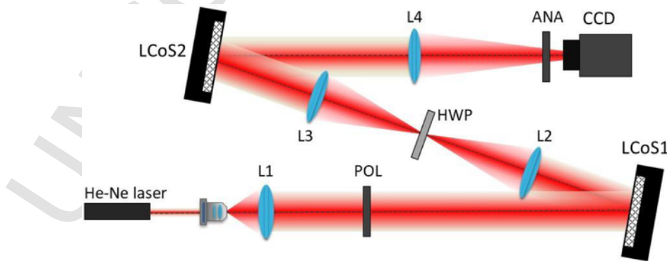
Fig. 1. Scheme of the optical setup. LCoS1 and LCoS2 are two liquid-crystal on silicon SLMs, with the liquid-crystal director oriented horizontally. A 4f -system (lenses L2 and L3) images LCoS1 onto LCoS2. POL: input linear polarizer. ANA: output polarization analyzer. HWP: half-wave plate. CCD: charge couple device detector.
