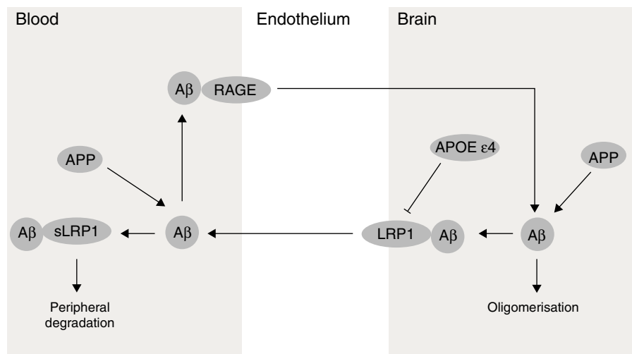
Figure 2 Regulatory mechanisms of A \beta levels in the brain parenchyma. APOE \epsilon 4: apolipoprotein \epsilon 4; LRP1: low-density lipoprotein 1 receptor; RAGE: receptor for advanced glycation end-products.
