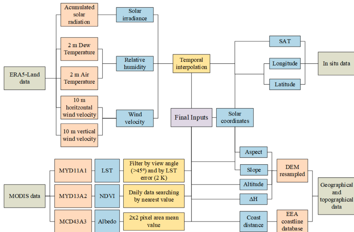
Fig. 3. Flowchart of data processing.
