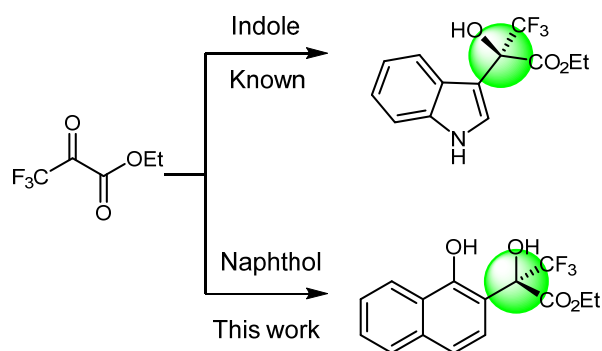
Scheme 1. Enantioselective Friedel-Crafts alkylation with ethyl trifluoropyruvate.
