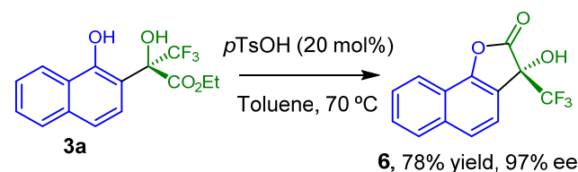
Scheme 3. Lactonization of 3a .
