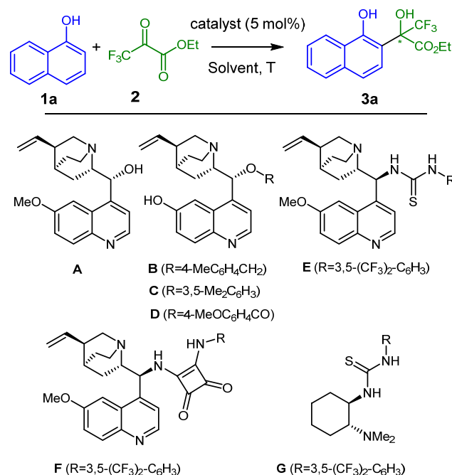
Scheme 1. Enantioselective Friedel-Crafts alkylation with ethyl trifluoropyruvate.
