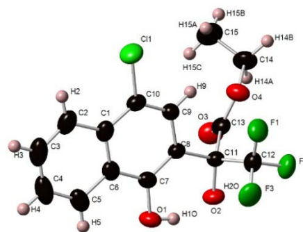
Figure 2. X-ray crystal structure of 3c .
