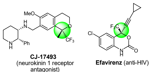
Figure 1. Structures of drugs containing a chiral tetrasubstituted carbon bearing a trifluoromethyl group.
