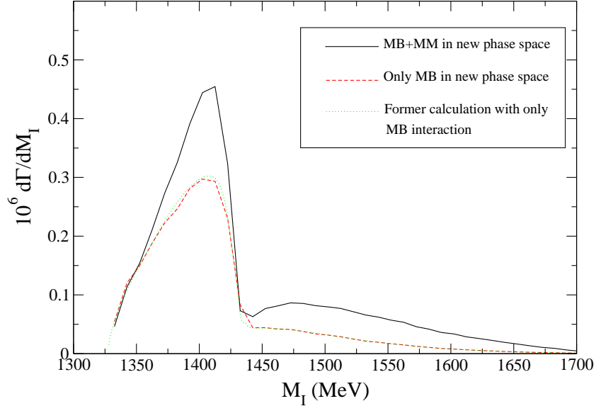
Figure 5: (Color online) The \pi\Sigma invariant mass distribution of the J/\psi \rightarrow \bar{\Sigma}^0\pi^0\Sigma^0\pi^0 channel calculated in new phase space of eq. 13 with Monte Carlo method. Solid line: the result in new phase space considering both meson baryon and meson meson interactions; Dashed line: the result in new phase space considering only meson baryon interactions; Dotted line: the result calculated with eq. (8) considering only meson baryon interaction.
