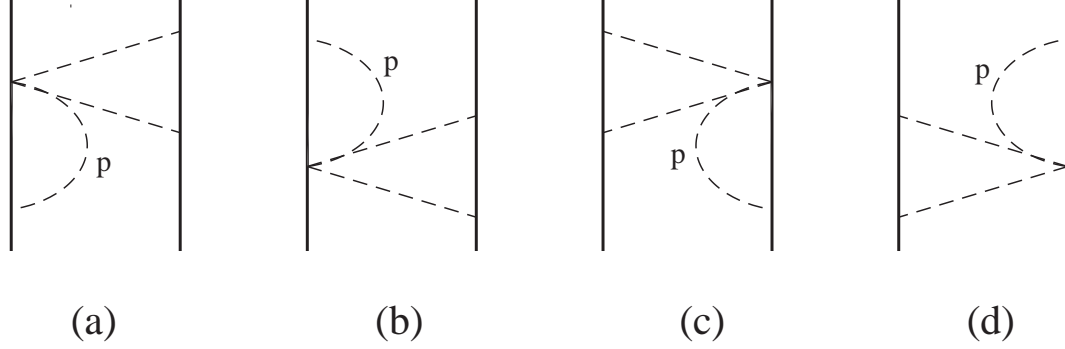
Figure 2: The processes with three meson vertex at a baryon line for pp \rightarrow pp .
