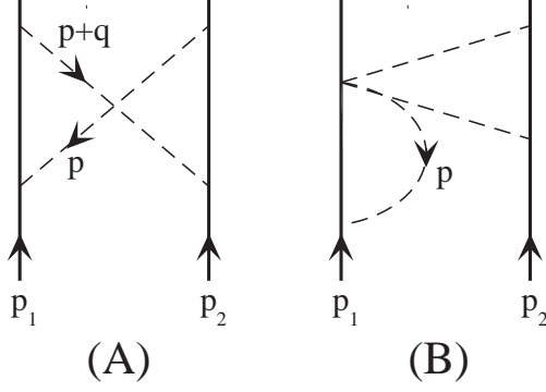
Figure 4: Diagrams where off-shell cancellations appear. Diagram (A) with the off shell part of the \pi \pi amplitude from the line p + q cancels diagram (B).
