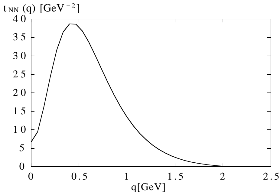
Figure 9: The function t_{NN} .
