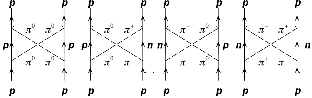
Figure 1: The lowest-order processes in the \pi\pi interaction in the scalar isoscalar channel for pp \rightarrow pp
