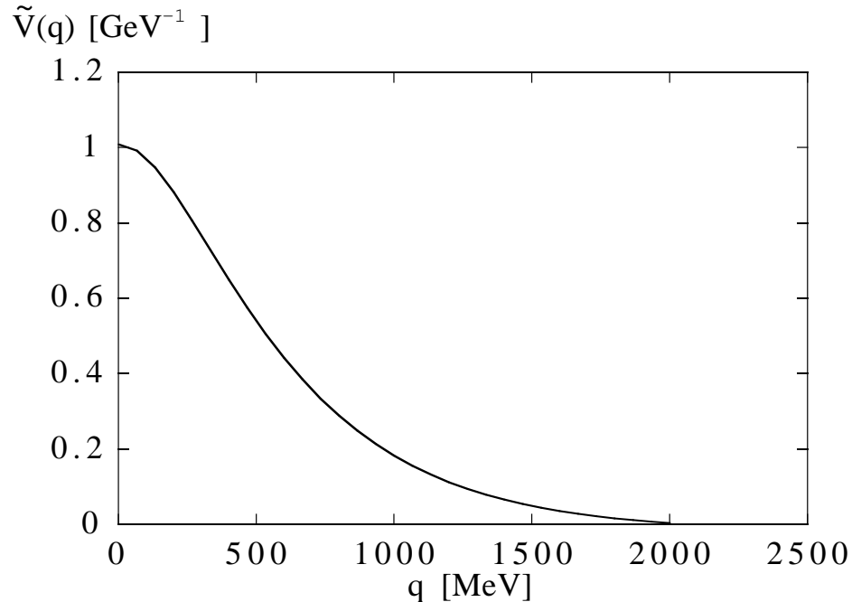
Figure 8: The vertex function \tilde{V}(q) as a function of momentum q .
