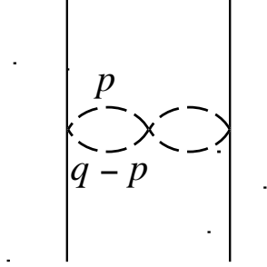
Figure 6: The nucleon-nucleon interaction with the two-pion nucleon vertex in the isoscalar channel.
