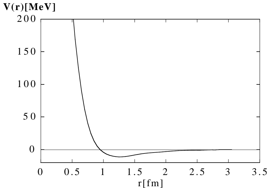
Figure 10: The NN potential in coordinate space
