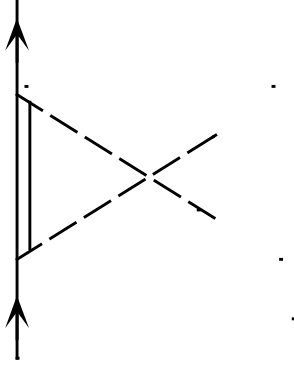
Figure 7: The two pion exchange triangle vertex through delta excitation.
