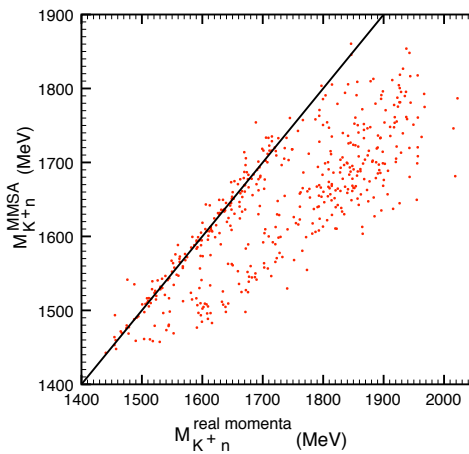
FIG. 1. M_{K^+n} calculated using the MMSA prescription versus M_{K^+n} obtained with the real momenta for the nucleons and the full model, i.e., \phi production on the nucleons and \Lambda(1520) production on the proton.
