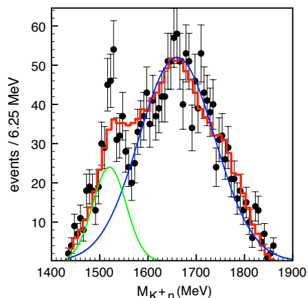
FIG. 3. M_{K^+n} invariant mass distribution obtained with the MMSA prescription and same cuts than LEPS normalized to the data of [4] (shown as dots), together with two gaussian functions: one peaking at 1520 MeV with a width of 80 MeV and another one peaking at 1660 MeV with a width of 185 MeV.
