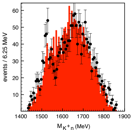
FIG. 5. M_{K^+n} invariant mass distribution calculated with \sim 2000 events, the MMSA prescription and the cut M_{K^+K^-} > 1030 MeV compared with the data of [4] (shown as dots).
