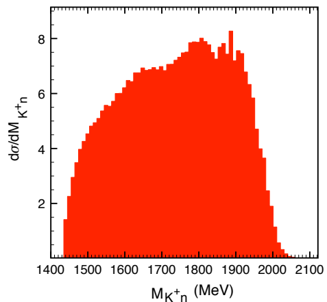
FIG. 2. M_{K^+n} invariant mass distribution calculated using the real momenta and with a \phi cut of M_{K^+K^-} > 1050 \text{ MeV} .
