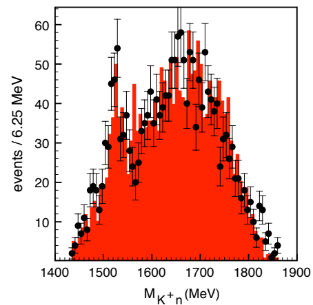
FIG. 6. M_{K^+n} invariant mass distribution calculated with \sim 2000 events, the MMSA prescription and the same cuts as those made in [4] compared with the data of [4] (shown as dots).
