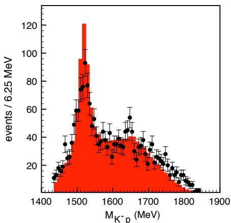
FIG. 4. M_{K^-p} invariant mass distribution calculated with the MMSA prescription and same cuts than LEPS normalized to the data of [4] (shown as dots).
