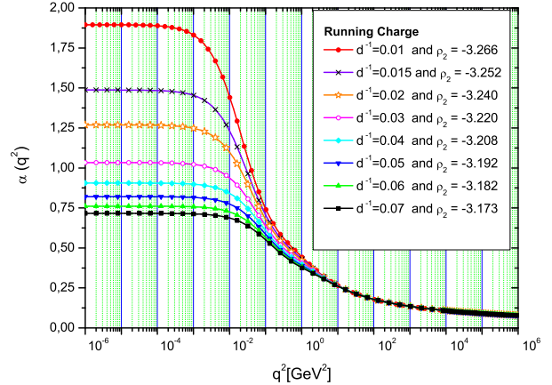
Fig. 3. The running charge, \alpha(q^2) , corresponding to the gluon propagator of Fig.(2).
