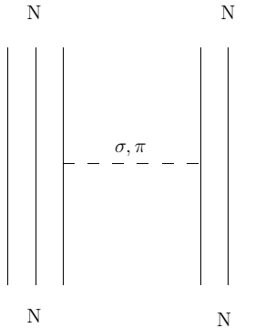
FIG. 1: Asymptotic NN OPE or OSE interactions at quark level.
