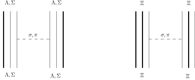
FIG. 4: Asymptotic \Lambda\Lambda , \Sigma\Sigma , and \Xi\Xi OPE and OSE interactions at quark level. Thin lines stand for light ( u, d ) quarks and thick lines for strange ( s ) quarks.
