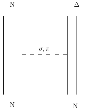
FIG. 3: Asymptotic NN \rightarrow N\Delta OPE or OSE interactions at quark level.
