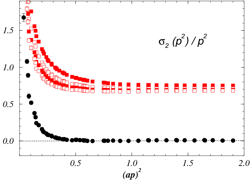
Figure 3: The effect of subtraction of the contact term, \tilde{c}'_q , from the scalar part of the quark propagator. Squares denote \sigma_2/p^2 , as obtained from unsubtracted (albeit corrected by the (1 + z^2 p^2) factor) propagators corresponding to the four values of the hopping parameters used in this study. The filled symbols denote \tilde{\sigma}_2/p^2 , obtained after the subtraction of the term due to \tilde{c}'_q (see Eq. (26) ), and extrapolated to the chiral limit.
