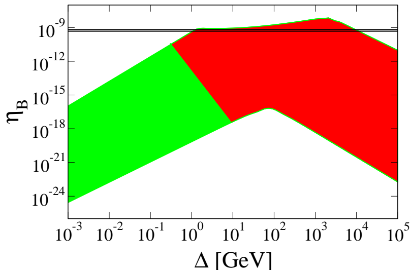
FIG. 8: Calculated range for \eta_B as a function of \Delta , for the ansatz defined in fig. (5), to the left. The horizontal band is the allowed range of \eta_B . The full shaded region corresponds to the allowed range without the sphaleron constraint, while the superimposed darker/red area indicates the allowed range of parameters once the sphaleron constraint is included. For a discussion see text.
