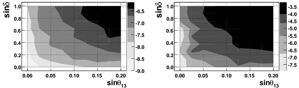
FIG. 6: Contours of the maximum value of the asymmetry obtained using the Fritzsche texture. Left panel: \tilde{F} = \tilde{f}Y , F symmetric. Right panel: \tilde{F} diagonal and F = X\tilde{F} .
