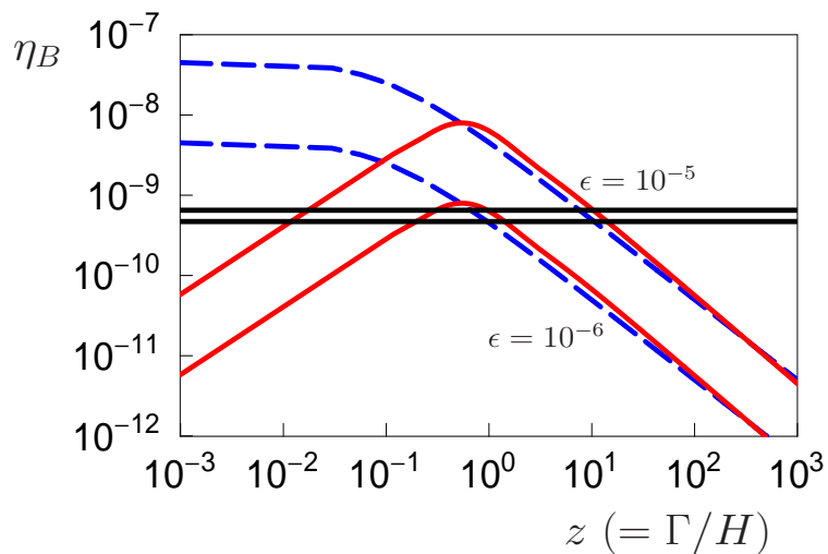
FIG. 7: Calculated range for \eta_B as a function of z , for the different fits to the washout factor. The dashed (full) lines show the approximate analytical solutions to the Boltzmann equations, see eqs (57) and (58). Results are shown for 2 typical values of \epsilon = 10^{-5}, 10^{-6} . The horizontal black band is the currently allowed \eta_B range [37].
