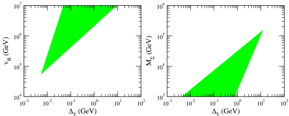
FIG. 3: v_R , M_\Sigma and \Delta_\Sigma values that follow from our first ansatz Eq. (49) for \tilde{f} = 0.1 , when the parameters are varied as in Eq. (53), see text.
