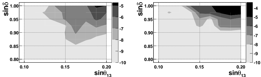
FIG. 5: Contour levels of the maximum asymmetry obtained as a function of \sin\theta_{13} and \sin\delta using the Fritzsche texture with \tilde{F} = X^{-1}F , F=I (left panel) or F symmetric (right panel).
