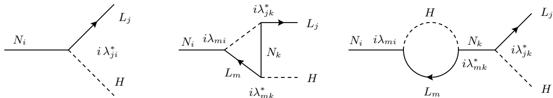
FIG. 1: Diagrams contributing to generate a lepton asymmetry of the universe.
