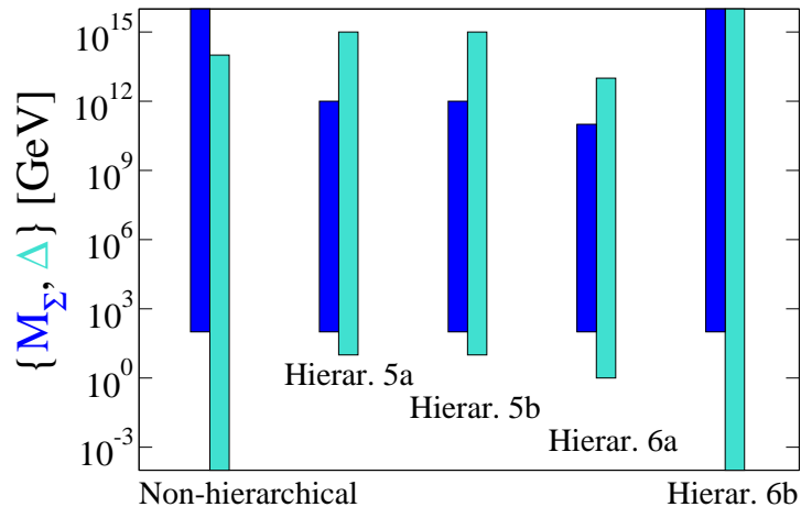
FIG. 9: Calculated ranges for \Delta and M_\Sigma for the different texture ansätze discussed in the text. This ranges have been obtained with the largest possible scan for the parameters, for example, M_\Sigma in the full interval [10^2, 10^{16}] GeV.
