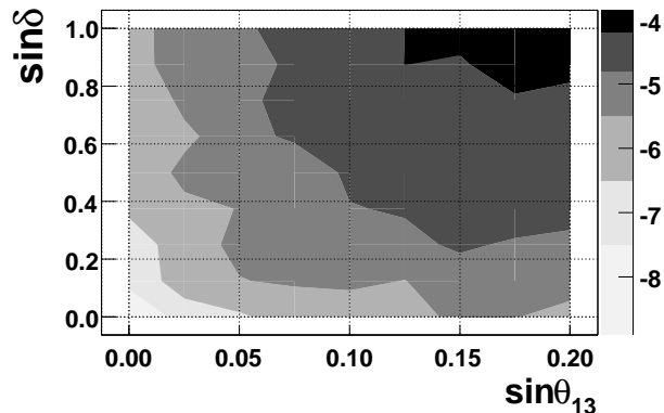
FIG. 4: Contour levels of the logarithm of the maximum value of the asymmetry \epsilon_\Sigma obtained as a function of \sin\theta_{13} and \sin\delta for the non-hierarchical ansatz of section IV A. The other neutrino mixing parameters are taken from the latest neutrino oscillation data given in [1].
