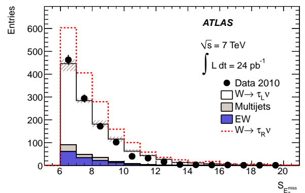
(b) Missing transverse momentum significance
