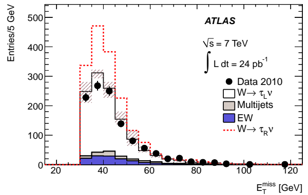
(a) Missing transverse momentum
