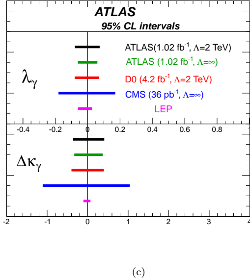
FIG. 4. The 95% CL intervals for anomalous couplings from ATLAS, D0 [3], CDF [1], CMS [5] and LEP [6] for (a),(b) the neutral aTGCs h_3^\gamma , h_3^Z , h_4^\gamma , h_4^Z as obtained from Z\gamma events, and (c) the charged aTGCs \Delta\kappa_\gamma , \lambda_\gamma . Integrated luminosities and new physics scale parameter \Lambda are shown. The ATLAS, CMS and Tevatron results for the charged aTGCs are measured from W\gamma production. The LEP charged aTGC results are obtained from WW\gamma production, which is sensitive also to the WWZ couplings and hence required some assumptions about the relations between the WW\gamma and WWZ aTGCs [6, 35–37]. The sensitivity of the LEP data to neutral aTGCs is much smaller than that of the hadron colliders; therefore the LEP results have not been included in (a) and (b).
