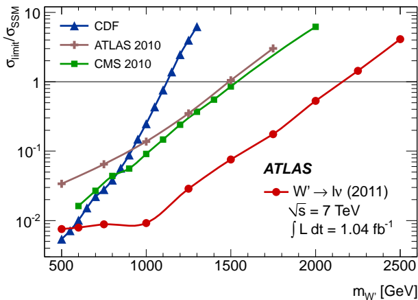
Figure 3: Normalized cross section limits ( \sigma_{\text{limit}}/\sigma_{\text{SSM}} ) for W' \rightarrow \ell\nu as a function of mass for this measurement and from CDF [2], CMS [3] and the previous ATLAS search [4]. The cross section calculations assume the W' has the same couplings as the standard model W boson. The region above each curve is excluded at the 95% CL.
