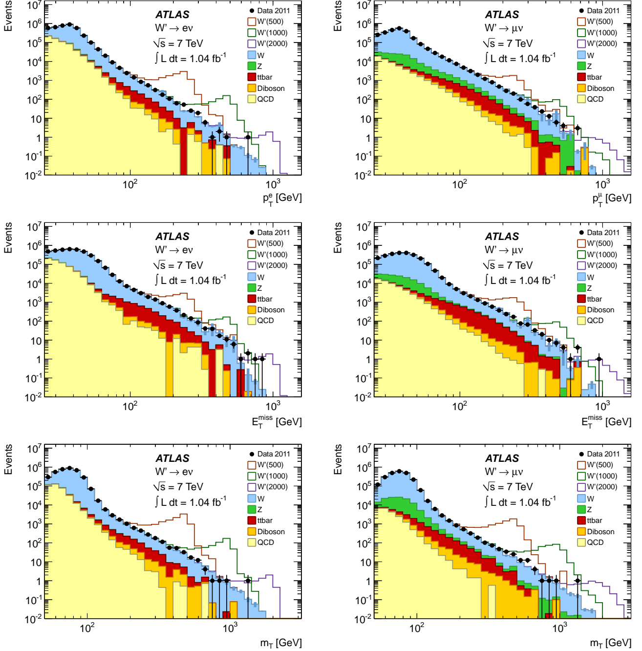
Figure 1: Spectra of p_T (top), missing E_T (center) and m_T (bottom) for the electron (left) and muon (right) channels after event selection. The points represent data and the filled histograms show the stacked backgrounds. Open histograms are W' \rightarrow l\nu signals added to the background with masses in GeV indicated in parentheses in the legend. The QCD backgrounds estimated from data are also shown. The signal and other background samples are normalized using the integrated luminosity of the data and the NNLO (approximate-NNLO for t\bar{t} ) cross sections listed in Table 1.
