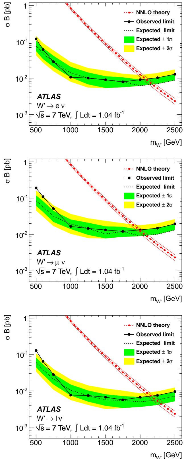
Figure 2: Expected and observed limits on \sigma B for W' \rightarrow e\nu (top), W' \rightarrow \mu\nu (center), and the combination (bottom) assuming the same branching fraction for both channels. The NNLO calculated cross section and its uncertainty are also shown.
