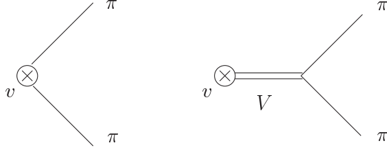
Figure 1: Tree-level contributions to the vector form factor of the pion. A single line stands for a pseudo-Goldstone boson while a double line indicates a vector resonance.
